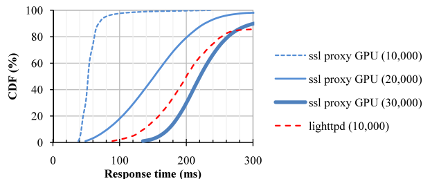
Figure 1: Response time distribution (Number in the parenthesis indicates offered load in HTTPS requests per seconds)
